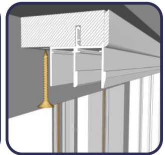
Reveal Fix
