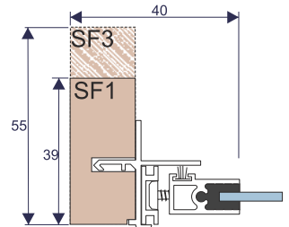
Luxury Subframe
