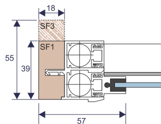
Luxury Subframe
